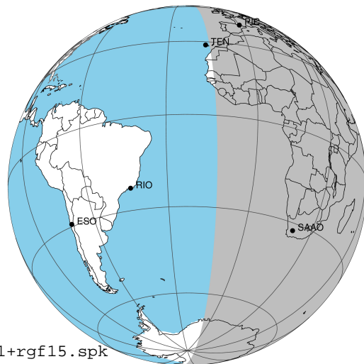
2043-09-28T18:45:22.6200 a: 17 40 03.1604 s: -23 15 30.294 C/A ***** PA 183.06 deg v_sky +18.02 km/s D 05.30 AU Credit: Styled after SORA/Lucky Star
