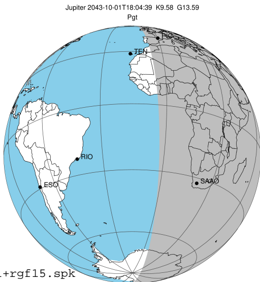
2043-10-01T18:04:39.4000 a: 17 41 33.1386 s: -23 16 42.329 C/A ***** PA 182.83 deg v_sky +19.35 km/s D 05.35 AU Credit: Styled after SORA/Lucky Star
