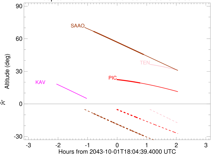
Jupiter 2043-10-01T18:04:39 K9.58 G13.59
