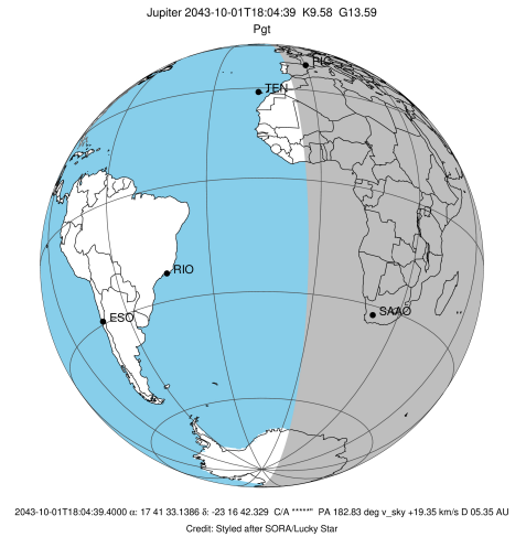
Jupiter 2043-10-01T18:04:39 K9.58 G13.59
