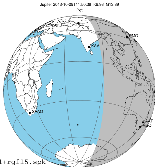
2043-10-09T11:50:39.5500 @: 17 45 53.4027 @: -23 19 18.049 C/A ***** PA 182.23 deg v_sky +22.71 km/s D 05.46 AU Credit: Styled after SORA/Lucky Star
