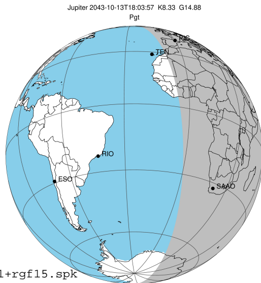
2043-10-13T18:03:57.9700 α: 17 48 31.5021 δ: -23 21 06.135 C/A ***** PA 1.89 deg v_sky +24.48 km/s D 05.52 AU Credit: Styled after SORA/Lucky Star
