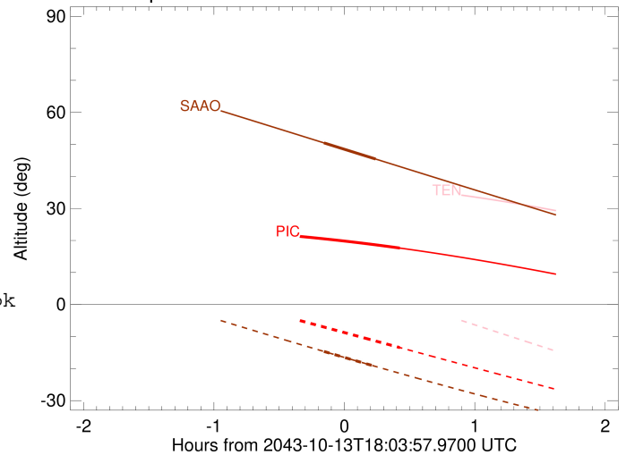
Jupiter 2043-10-13T18:03:57 K8.33 G14.88
