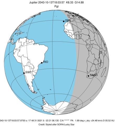
Jupiter 2043-10-13T18:03:57 K8.33 G14.88
