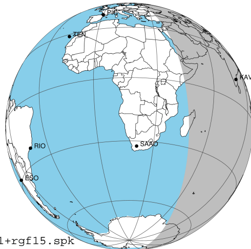
2043-10-21T14:49:33.5900 α: 17 53 49.0810 δ: -23 23 08.256 C/A ***** PA 1.26 deg v_sky +27.58 km/s D 05.63 AU Credit: Styled after SORA/Lucky Star
