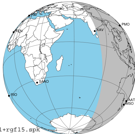
2043-10-22T12:09:45.5800 α: 17 54 26.9878 δ: -23 22 48.544 C/A ***** PA 181.20 deg v_sky +27.92 km/s D 05.64 AU Credit: Styled after SORA/Lucky Star
