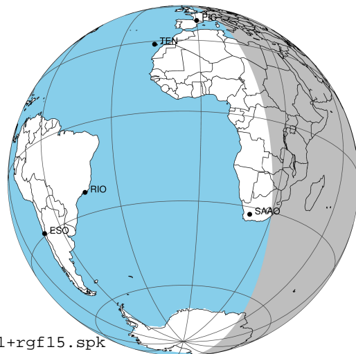
2043-10-23T16:13:11.5800 α: 17 55 17.3333 δ: -23 23 18.032 C/A 3.529" PA 1.10 deg v_sky +28.36 km/s D 05.66 AU Credit: Styled after SORA/Lucky Star
