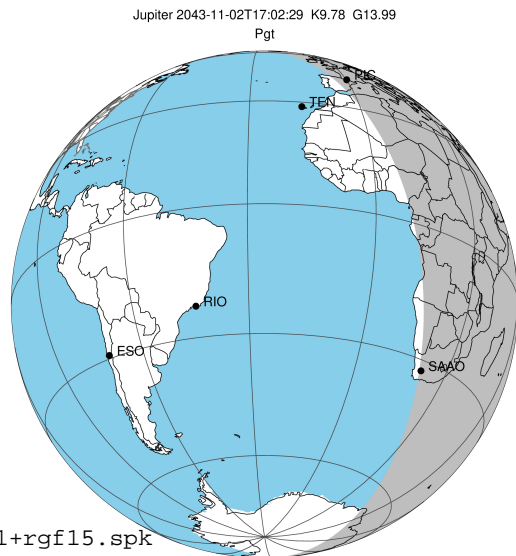
2043-11-02T17:02:29.1300 ex: 18 02 55.4462 s: -23 24 23.967 C/A 4.924" PA 180.26 deg v_sky +31.97 km/s D 05.78 AU Credit: Styled after SORA/Lucky Star
