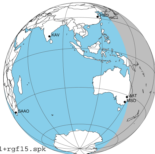
2043-11-05T08:18:10.3700 ± 18 05 02.9030 ± -23 24 22.735 C/A ***** PA 180.03 deg v_sky +32.84 km/s D 05.81 AU Credit: Styled after SORA/Lucky Star
