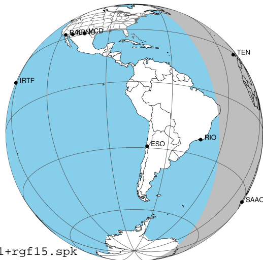
2043-11-05T20:17:09.2000 ca: 18 05 27.3541 s: -23 24 27.516 C/A 5.731" PA 179.98 deg v_sky +33.00 km/s D 05.82 AU Credit: Styled after SORA/Lucky Star
