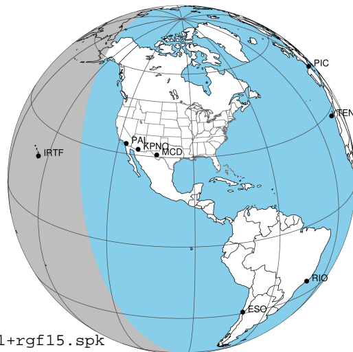
2048-08-10T14:33:08.5600 α: 05 31 37.8409 δ: +22 44 42.320 C/A ***** PA 357.05 deg v_sky +29.97 km/s D 05.58 AU Credit: Styled after SORA/Lucky Star
