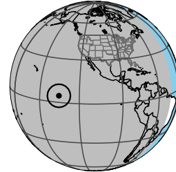
2042-09-23T02:01:31 K12.56 G14.29 PRt
