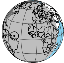
2046-10-04T02:46:40 K14.57 G17.44 PgtRgt
