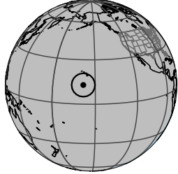
2045-09-09T04:55:25 K14.21 G17.95 PgtRgt
