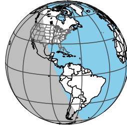
2042-09-15T05:36:33 K14.51 G15.65 PgtRgt
