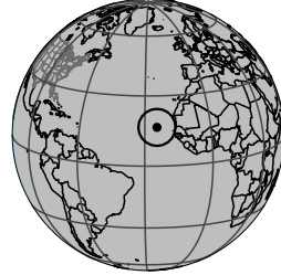
2046-01-31T07:17:34 K10.53 G12.50 PgtX
