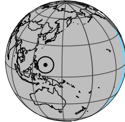
2046-10-21T14:49:48 K13.56 G17.42 PgtRgt
