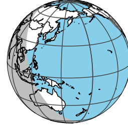
2047-02-22T10:11:34 K13.83 G17.60 PgtRgt
