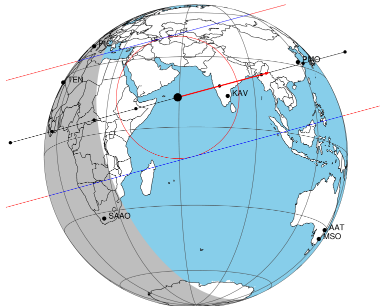
2023-04-20T04:10:03.0300 α: 22 26 36.3992 δ: -11 14 33.156 C/A 0.345" PA 344.78 deg v_sky +30.34 km/s D 10.35 AU Credit: Styled after SORA/Lucky Star
