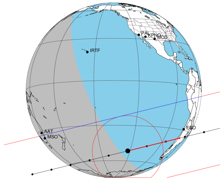
2024-05-21T16:27:38.1700 α: 23 18 10.6474 δ: -06 28 24.517 C/A 0.629" PA 166.17 deg v_sky +23.80 km/s D 09.95 AU Credit: Styled after SORA/Lucky Star
