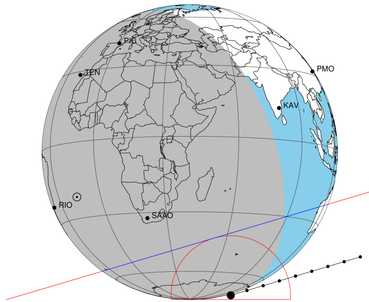
2024-07-16T01:03:32.7200 cc: 23 22 17.8358 s: -06 17 20.386 C/A 0.979" PA 163.45 deg v_sky -12.14 km/s D 09.06 AU
