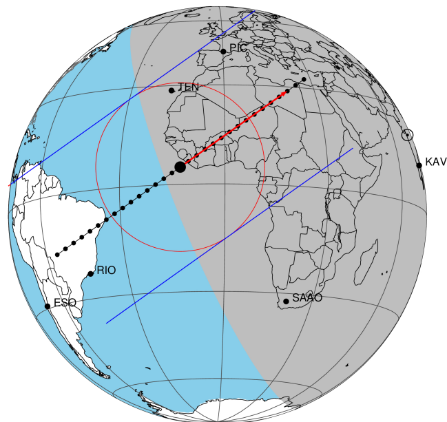
2024-11-24T18:50:40.7000 α: 22 58 10.0059 δ: -08 48 46.412 C/A 0.272" PA 324.57 deg v_sky + 5.13 km/s D 09.43 AU Credit: Styled after SORA/Lucky Star
