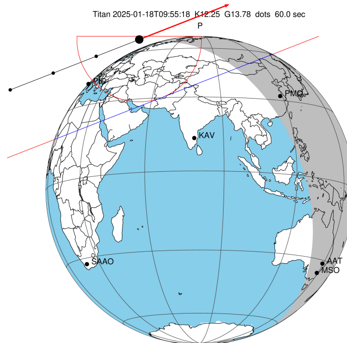
2025-01-18T09:55:18.4300 α: 23 10 29.0345 δ: -07 26 20.255 C/A 0.904" PA 338.66 deg v_sky +31.80 km/s D 10.27 AU Credit: Styled after SORA/Lucky Star
