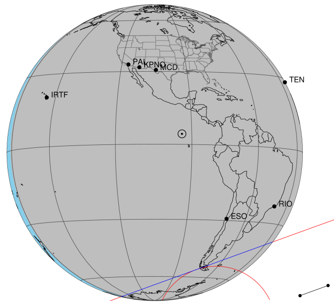
2025-10-03T06:04:39.9300 ra: 23 53 59.9428 s: -03 24 38.017 C/A 1.275" PA 160.14 deg v_sky -21.40 km/s D 08.56 AU Credit: Styled after SORA/Lucky Star
