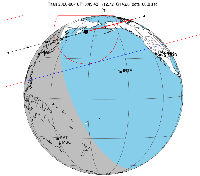
2026-06-10T18:49:43.3100 α: 00 50 05.8871 δ: +02 52 13.397 C/A 0.738" PA 344.98 deg v_sky +26.80 km/s D 09.83 AU Credit: Styled after SORA/Lucky Star
