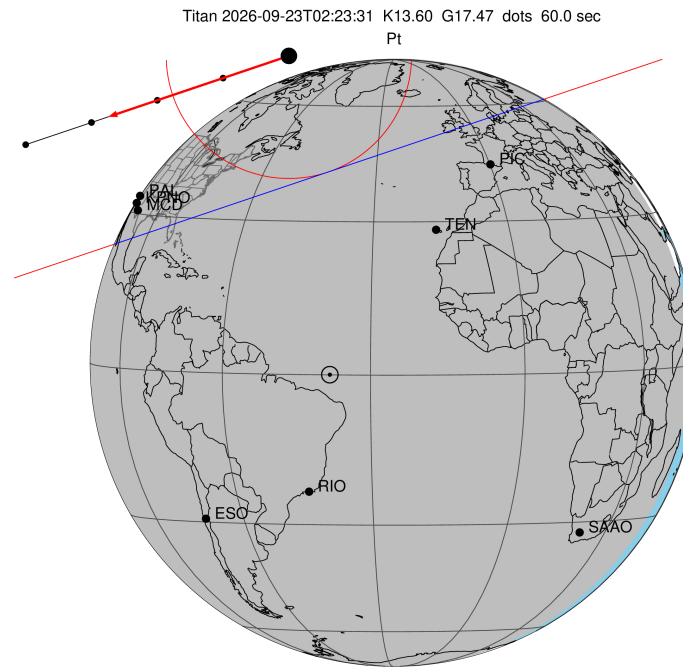
2026-09-23T02:23:31.4800 α: 00 47 37.0647 δ: +02 11 09.394 C/A 1.113" PA 341.35 deg v_sky -24.30 km/s D 08.45 AU Credit: Styled after SORA/Lucky Star
