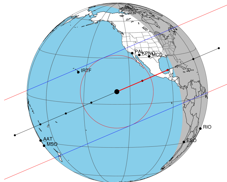
2028-02-25T23:45:34.3800 α: 01 32 51.4101 δ: +07 11 01.737 C/A 0.012" PA 336.34 deg v_sky +32.58 km/s D 09.93 AU Credit: Styled after SORA/Lucky Star
