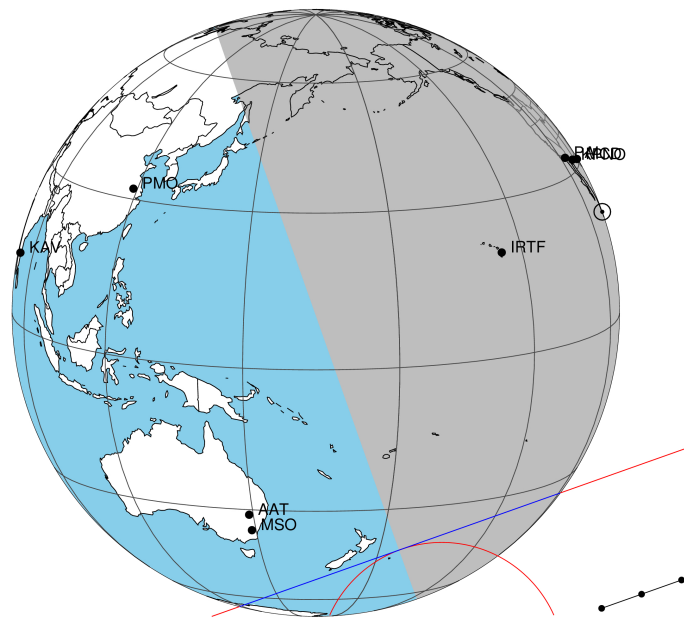
2029-01-24T07:01:49.9200 α: 02 11 39.0671 δ: +10 41 42.117 C/A 1.184" PA 160.48 deg v_sky +14.83 km/s D 09.15 AU Credit: Styled after SORA/Lucky Star
