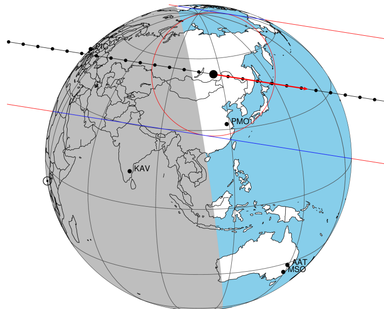
2030-09-03T22:31:30.7200 cc: 04 27 08.2782 d: +19 43 14.674 C/A 0.543" PA 8.97 deg v_sky +10.29 km/s D 08.98 AU Credit: Styled after SORA/Lucky Star
