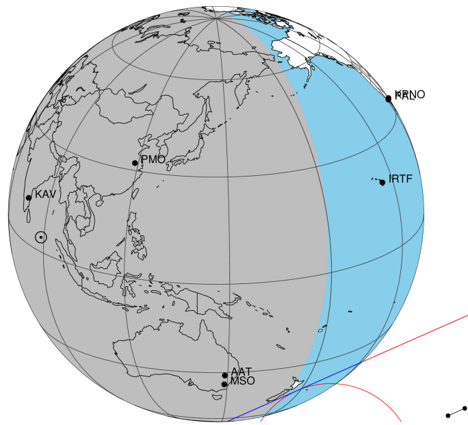
2030-10-03T17:54:29.5600 cc: 04 27 37.7937 d: +19 40 55.796 C/A 1.384" PA 156.16 deg v_sky - 9.35 km/s D 08.51 AU
