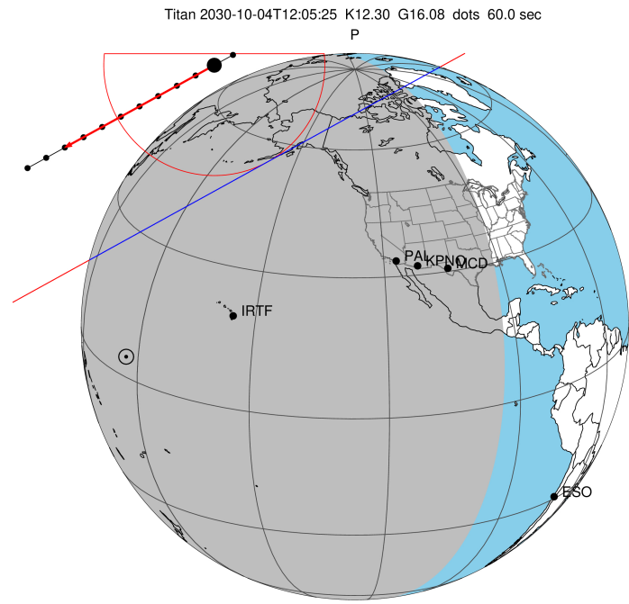
2030-10-04T12:05:25.9100 cc: 04 27 31.9151 d: +19 40 12.035 C/A 1.124" PA 331.13 deg v_sky - 8.29 km/s D 08.50 AU Credit: Styled after SORA/Lucky Star
