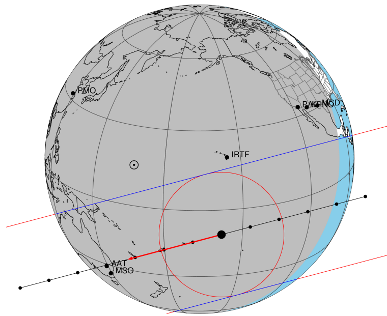
2030-11-04T12:33:09.4000 α: 04 21 10.7037 δ: +19 23 07.130 C/A 0.548" PA 165.15 deg v_sky -20.45 km/s D 08.16 AU Credit: Styled after SORA/Lucky Star
