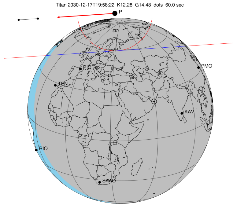
2030-12-17T19:58:22.4100 α: 04 07 20.7309 δ: +18 50 28.472 C/A 1.137" PA 356.13 deg v_sky -22.07 km/s D 08.14 AU Credit: Styled after SORA/Lucky Star
