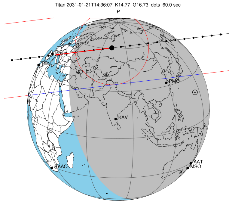
2031-01-21T14:36:07.8300 α: 03 59 48.2152 δ: +18 37 58.623 C/A 0.698" PA 352.97 deg v_sky -10.65 km/s D 08.51 AU Credit: Styled after SORA/Lucky Star
