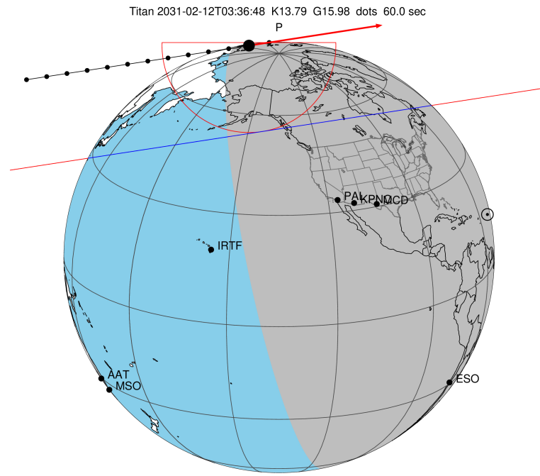
2031-02-12T03:36:48.2600 α: 03 59 37.7543 δ: +18 40 58.457 C/A 0.986" PA 351.27 deg v_sky +10.11 km/s D 08.86 AU Credit: Styled after SORA/Lucky Star
