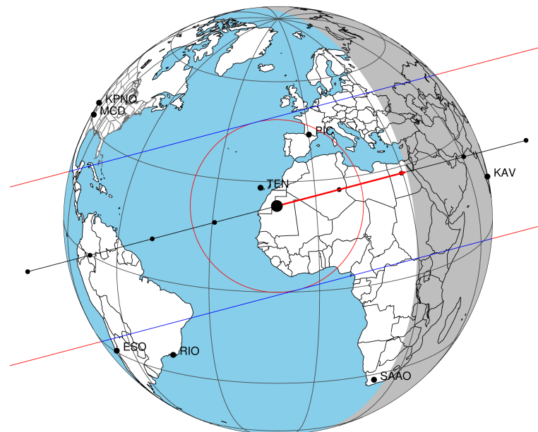
2031-04-04T16:08:22.5800 α: 04 12 59.3733 δ: +19 30 12.069 C/A 0.061" PA 345.09 deg v_sky +31.94 km/s D 09.66 AU Credit: Styled after SORA/Lucky Star
