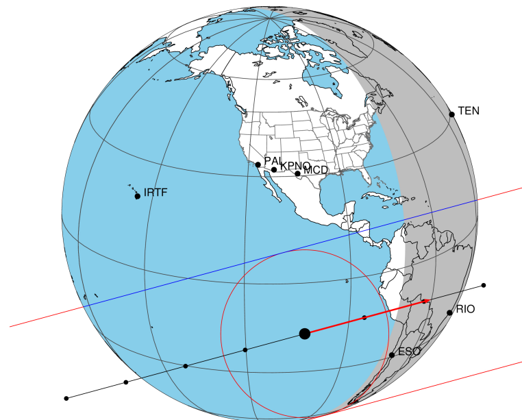
2031-04-04T22:54:32.7500 α: 04 13 06.9077 δ: +19 30 41.225 C/A 0.545" PA 164.82 deg v_sky +31.55 km/s D 09.66 AU Credit: Styled after SORA/Lucky Star
