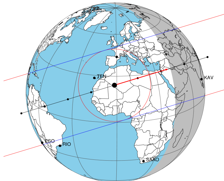
2031-04-06T15:20:29.5100 α: 04 13 49.5860 δ: +19 33 34.619 C/A 0.073" PA 343.18 deg v_sky +28.86 km/s D 09.68 AU Credit: Styled after SORA/Lucky Star
