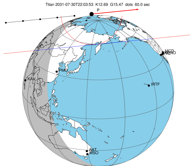
2031-07-30T22:03:53.4600 α: 05 12 17.6318 δ: +21 31 24.815 C/A 0.927" PA 354.24 deg v_sky +24.17 km/s D 09.68 AU Credit: Styled after SORA/Lucky Star
