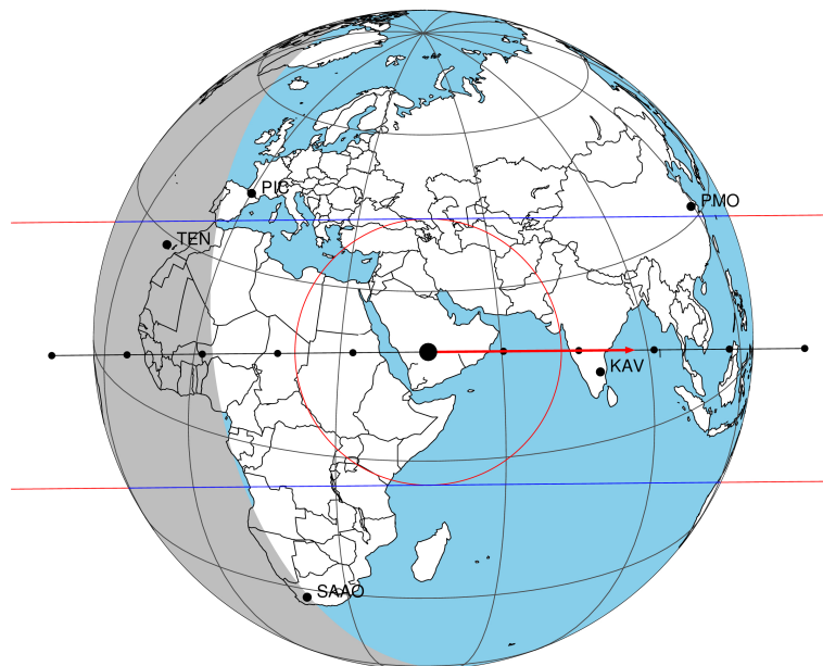
2031-08-02T05:30:40.5400 α: 05 13 06.1820 δ: +21 32 02.169 C/A 0.034" PA 179.31 deg v_sky +24.27 km/s D 09.65 AU Credit: Styled after SORA/Lucky Star
