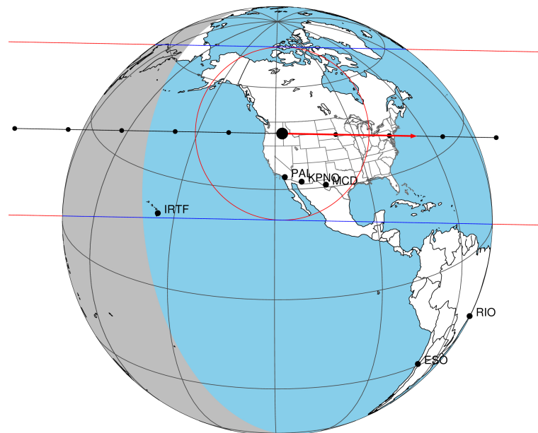
2031-08-03T16:24:13.2500 cc: 05 13 38.7058 & +21 31 58.137 C/A 0.373" PA 1.09 deg v_sky +26.45 km/s D 09.63 AU
