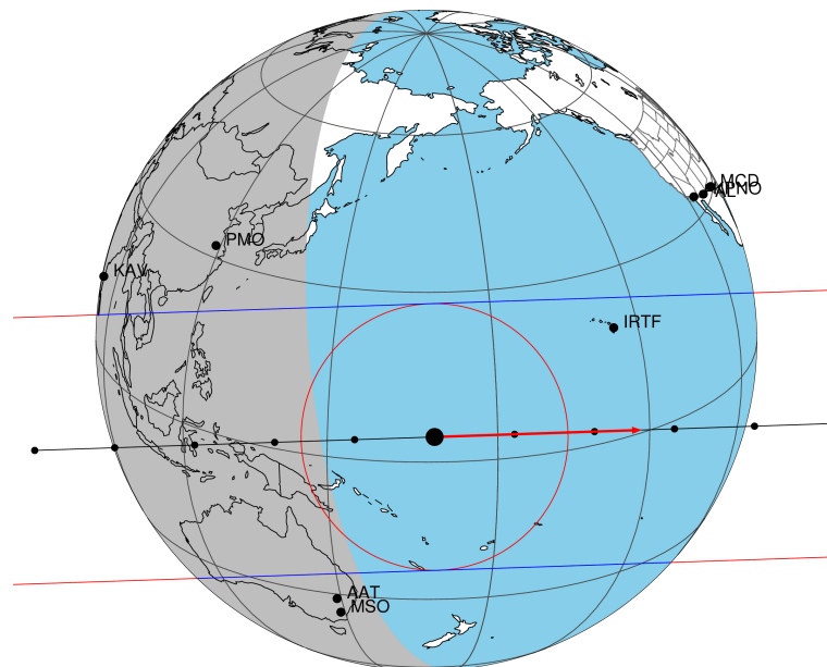
2031-08-23T20:05:23.9700 α: 05 21 09.1866 δ: +21 36 44.144 C/A 0.276" PA 178.06 deg v_sky +25.73 km/s D 09.35 AU Credit: Styled after SORA/Lucky Star
