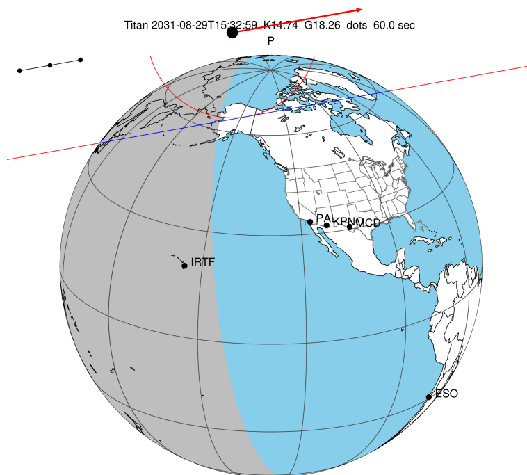
2031-08-29T15:32:59.2100 α: 05 23 04.7609 δ: +21 39 56.217 C/A 1.066" PA 349.82 deg v_sky +15.53 km/s D 09.25 AU Credit: Styled after SORA/Lucky Star
