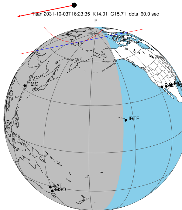
2031-10-03T16:23:35.5900 cc: 05 28 01.6358 s: +21 41 44.034 C/A 1.278" PA 348.51 deg v_sky - 4.80 km/s D 08.68 AU
