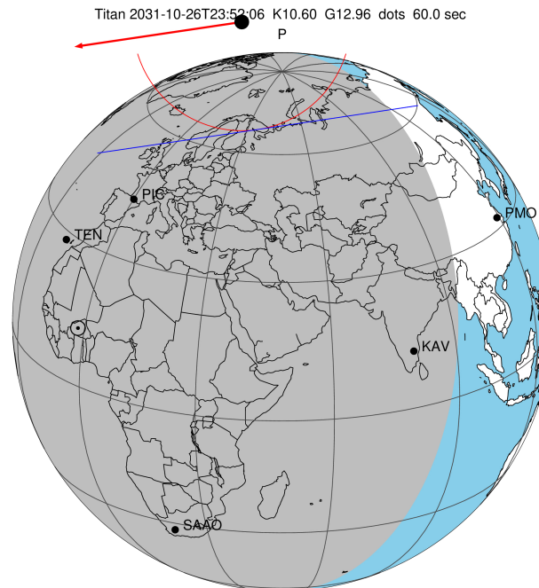
2031-10-26T23:52:06.4300 cc: 05 26 12.95812 s +21 35 38.369 C/A 1.182" PA 351.56 deg v_sky - 4.25 km/s D 08.36 AU Credit: Styled after SORA/Lucky Star
