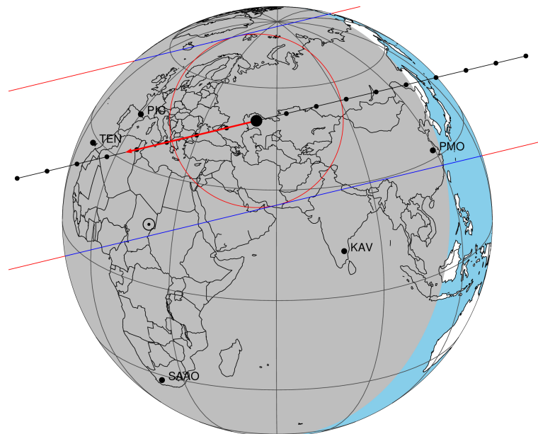
2031-11-07T22:16:39.8600 α: 05 23 31.3649 δ: +21 34 27.945 C/A 0.512" PA 346.45 deg v_sky -15.21 km/s D 08.22 AU
