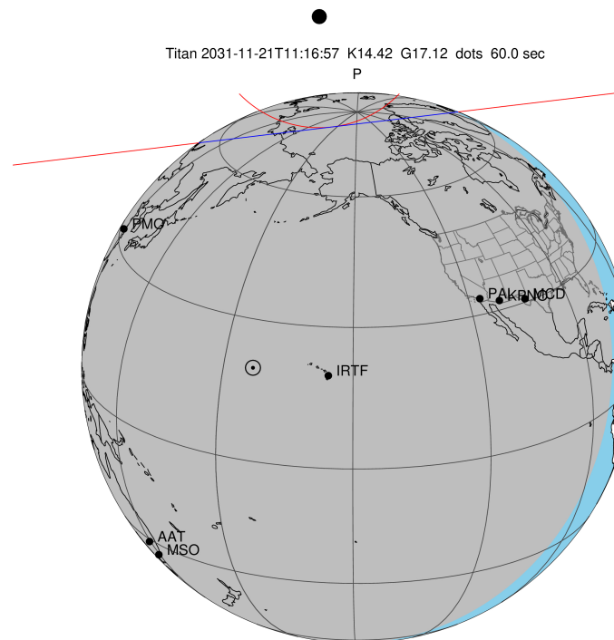
2031-11-21T11:16:57.2100 α: 05 19 49.7630 δ: +21 32 08.044 C/A 1.394" PA 353.18 deg v_sky -22.94 km/s D 08.10 AU Credit: Styled after SORA/Lucky Star
