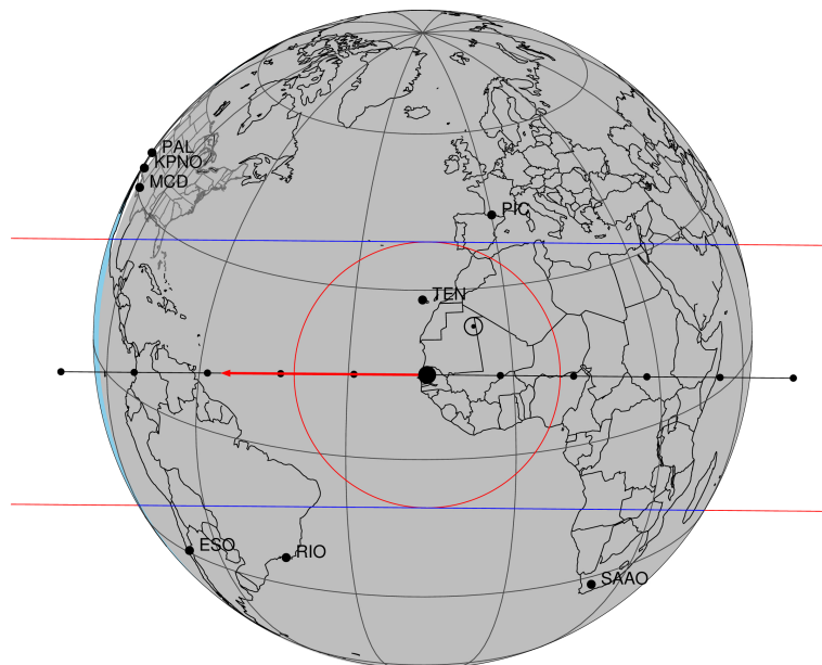
2031-12-20T00:24:27.5800 α: 05 10 18.2731 δ: +21 23 30.437 C/A 0.118" PA 180.50 deg v_sky -23.63 km/s D 08.05 AU Credit: Styled after SORA/Lucky Star
