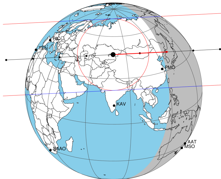
2032-04-17T10:15:01.1400 α: 05 11 45.4274 δ: +21 47 52.882 C/A 0.379" PA 357.10 deg v_sky +32.12 km/s D 09.62 AU Credit: Styled after SORA/Lucky Star
