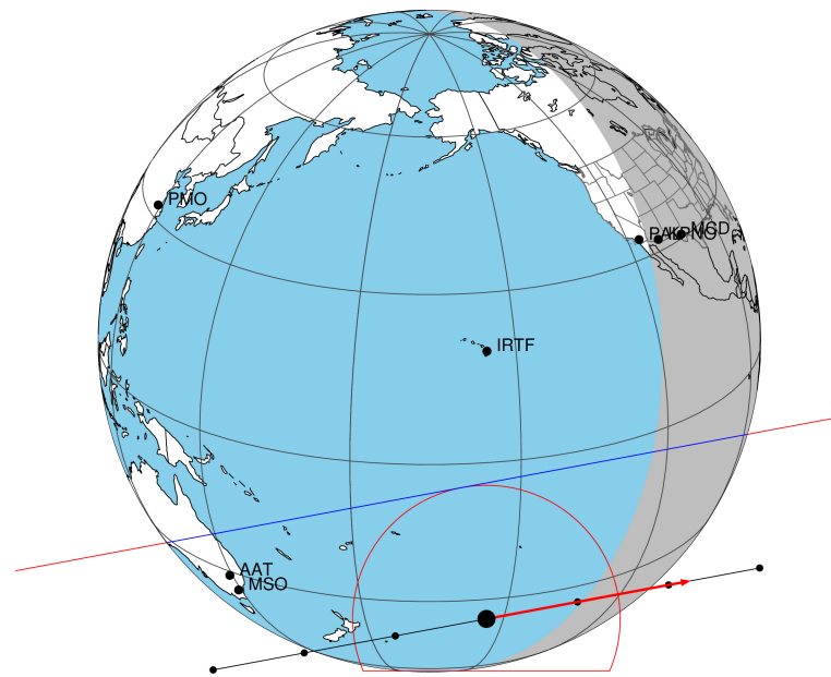
2032-04-24T02:10:34.5500 α: 05 14 59.4877 δ: +21 53 45.968 C/A 0.777" PA 169.42 deg v_sky +29.73 km/s D 09.69 AU Credit: Styled after SORA/Lucky Star
