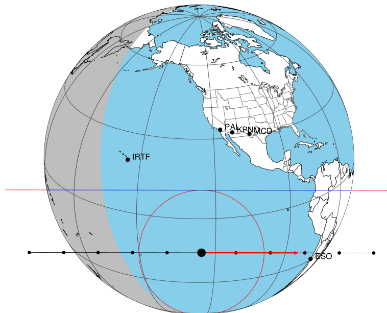
2032-08-16T16:58:51.8200 α: 06 14 32.1973 δ: +22 25 27.675 C/A 0.549" PA 180.09 deg v_sky +23.61 km/s D 09.62 AU Credit: Styled after SORA/Lucky Star
