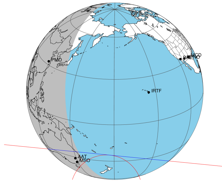
2032-08-22T20:10:12.4300 α: 06 16 45.9415 δ: +22 22 31.666 C/A 1.039" PA 185.67 deg v_sky +28.78 km/s D 09.55 AU Credit: Styled after SORA/Lucky Star
