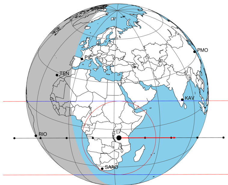
2032-08-26T05:51:53.2600 α: 06 18 18.8282 δ: +22 21 29.365 C/A 0.437" PA 179.81 deg v_sky +30.41 km/s D 09.50 AU Credit: Styled after SORA/Lucky Star
