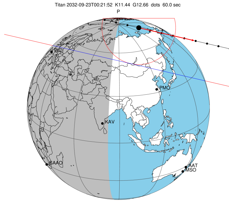
2032-09-23T00:21:52.3700 α: 06 26 11.9562 δ: +22 17 32.163 C/A 0.890" PA 13.09 deg v_sky +13.60 km/s D 09.07 AU Credit: Styled after SORA/Lucky Star
