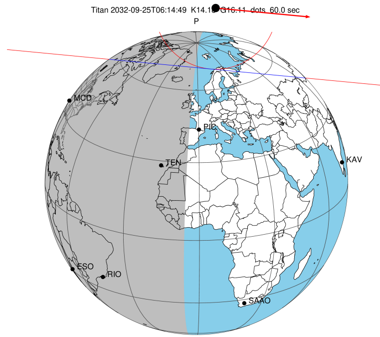
2032-09-25T06:14:49.2400 cc: 06 26 43.9066 â: +22 16 19.986 C/A 1.132" PA 5.44 deg v_sky +16.40 km/s D 09.03 AU Credit: Styled after SORA/Lucky Star
