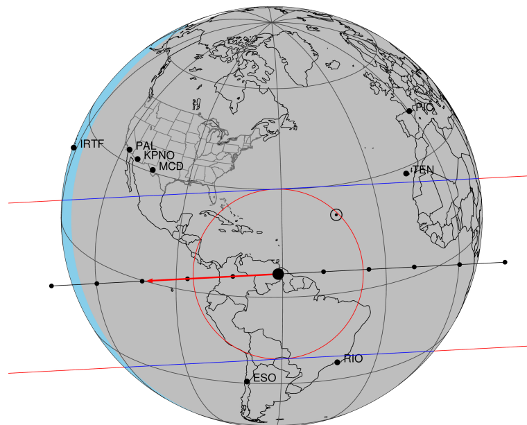
2033-01-10T03:02:11.3600 α: 06 08 08.2685 δ: +22 30 08.347 C/A 0.298" PA 176.99 deg v_sky -22.92 km/s D 08.07 AU Credit: Styled after SORA/Lucky Star
